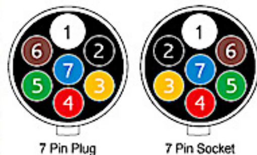
Cable Entry View
