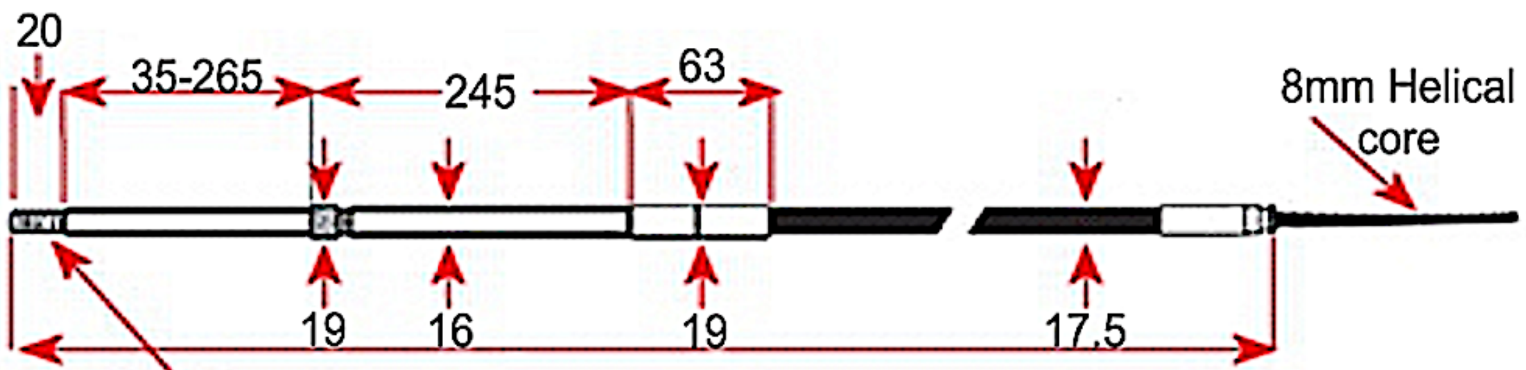
3/8" J-D0499 Cable Order Length at Mid Travel UNF
